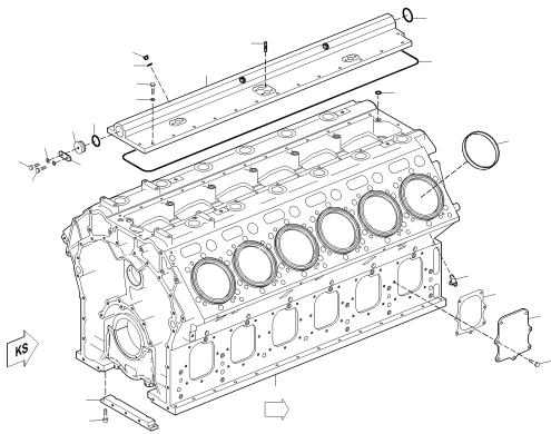
CRANKCASE UPC.06A01 2075
